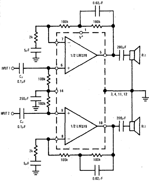
Simple Stereo Amplifier with Bass Boost
