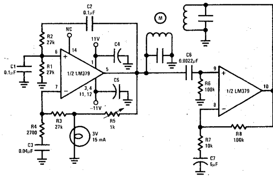
Two-Phase Motor Drive
