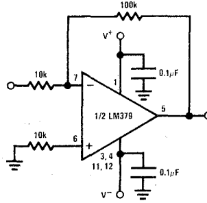
Power Op Amp (Using Split Supplies)
