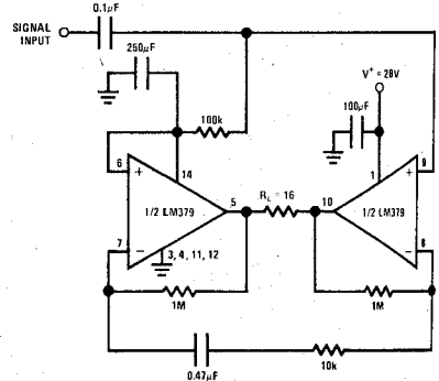
12W Bridge Amplifier
